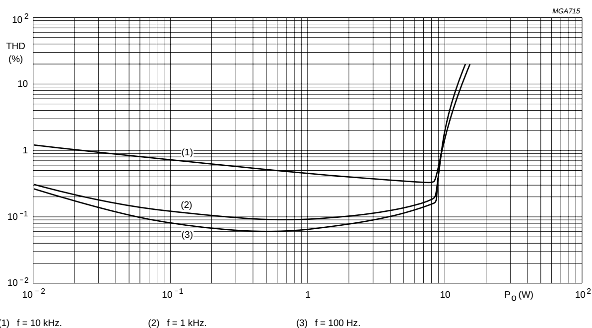
Fig.18 Total harmonic distortion as a function of output power; V_P = 14.4 \text{ V} , R_L = 2 \Omega .
